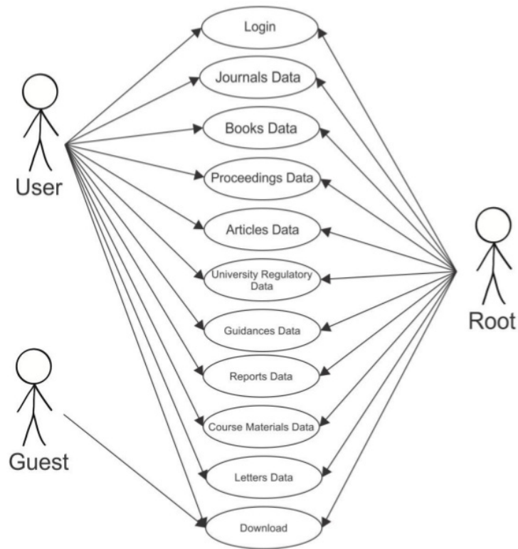
Figure 3. Repository Use case diagram
