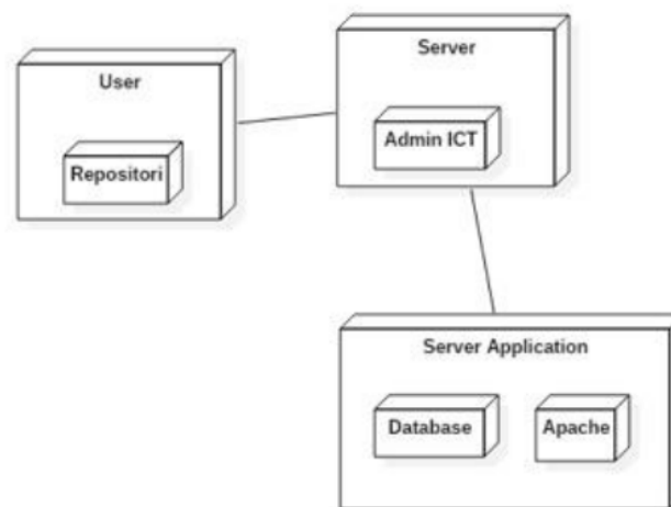
Figure 5. Repository Deployment
