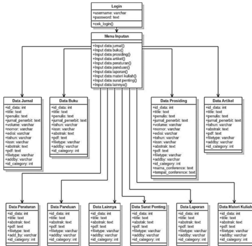
Figure 4. Repository Class diagram
