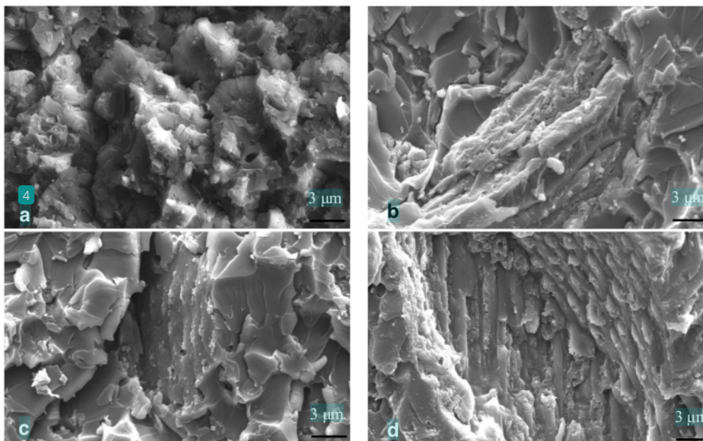
Fig. 7. SEM image of the carbon fiber of Jatropha seed shell filled vinyl ester composites: (a) Control (source: Sri Aprila et al. 2014) (b) after immersion in 5% NaOH for 12 months, (c) after immersion in 5% HCl for 12 months, and (d) after immersion in distilled water for 12 months
