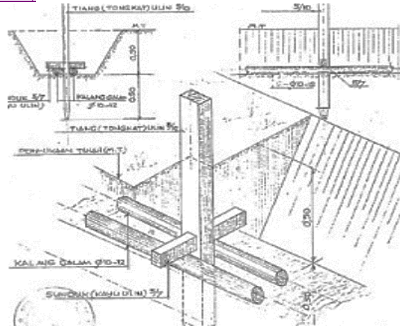
Figure 8: Wooden House Foundation
