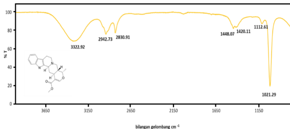
Gambar 3. Spektrum standar ajmalicine
