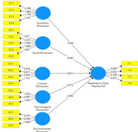
Figure 3: Bootstrapping Result
