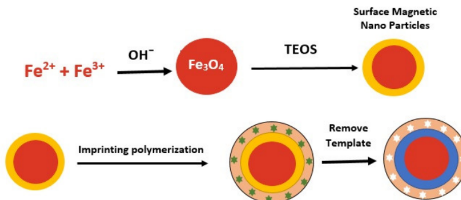
Figure 4. The preparation of MMIPs using silica.
