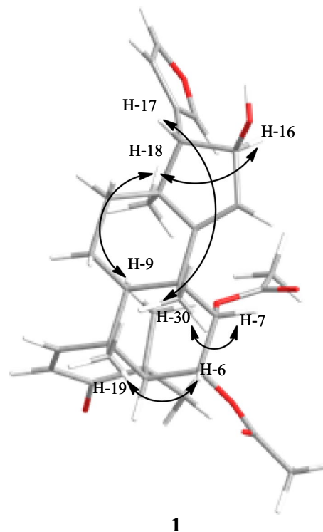
Fig. 3 Selected NOESY correlations for 1
