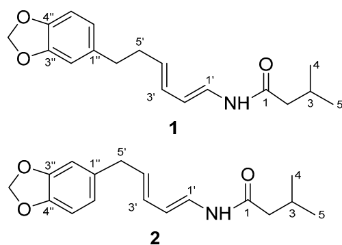
Figure 2. Structures of piperenamide A-B (1–2).
