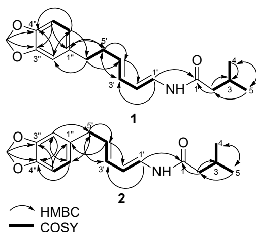
Figure 3. Selected HMBC and COSY correlations for piperenamides A-B (1–2).
