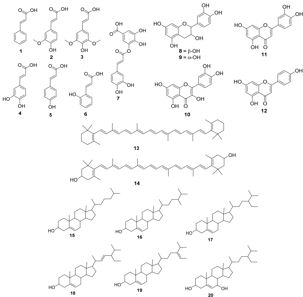
FIGURE 2. Structures of secondary metabolites present in date seed extract
