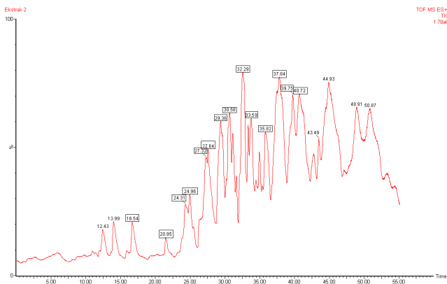
FIGURE 1. HPLC chromatogram of the P. dactylifera seed extract
