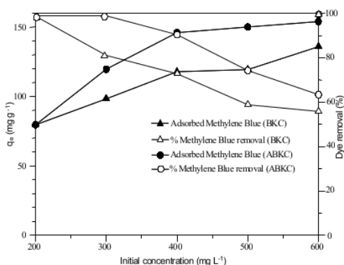
Figure 9. The effect of initial synthetic dye concentration.
