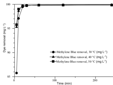
Figure 8. The effect of contact time on methylene blue removal on ABKC. Conditions: (pH: 6.9, MB: 100 \text{ mg}\cdot\text{L}^{-1} , weight of adsorbent: 62.5 mg, at 30, 40 and 50 °C).
