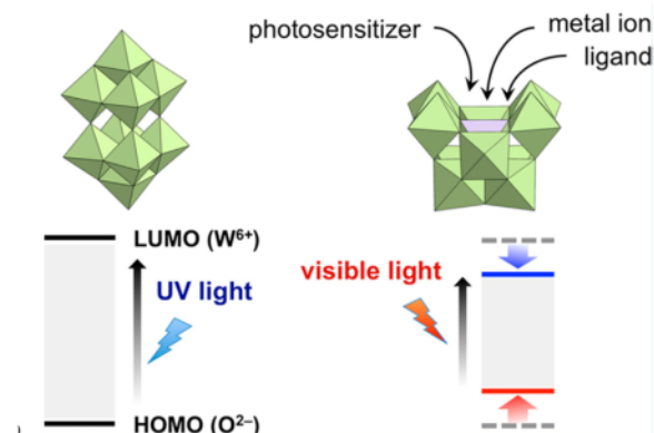
Fig. 8. UV responsive through charge transfer from the O_2 -based HOMOs and the W^{6+} -based LUMOs. Visible lights responsive POM catalysts through hybridization with photosensitizer, metal substitution, and introduction of ligands (substrates) at the vacant sites of lacunary POMs. Reprinted with permission from (Suzuki et al., 2018). Copyright 2018 American Chemical Society.
