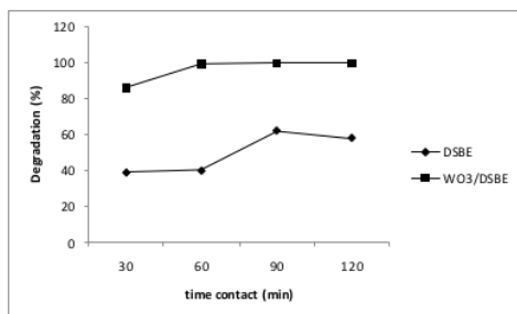
Figure 4. Contact time variations on degradation percentage.
