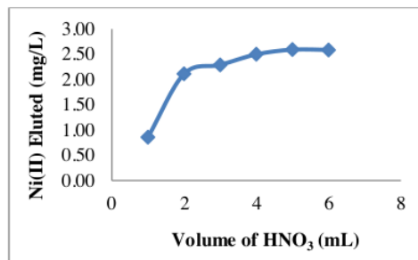
Figure 4. Effect of volume HNO 3 as eluent
