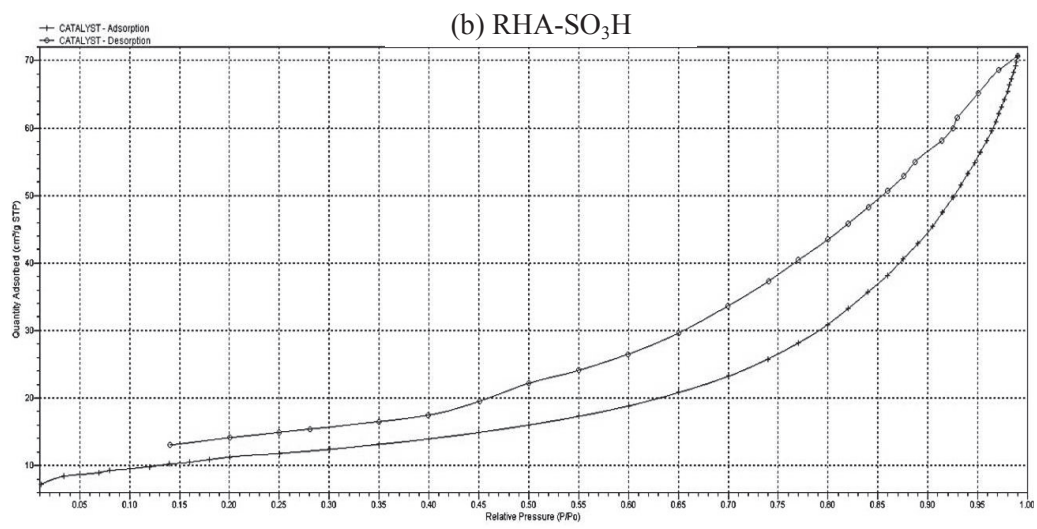
FIGURE 3. N 2 adsorption-desorption isotherms of RHA and RHA-SO 3 H
