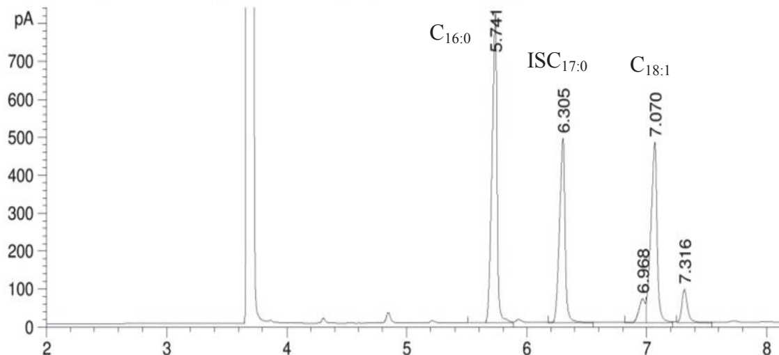
FIGURE 6. Gas Chromatogram of methyl ester from DC-oil
