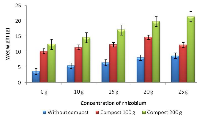
Figure 2. Effect of Rhizobium inoculant treatment on wet weight
