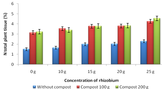
Figure 5. Effect of Rhizobium inoculant treatment on nitrogen concentration plant tissue
