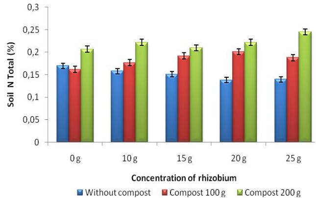
Figure 4. Effect of compost treatment on soil nitrogen
