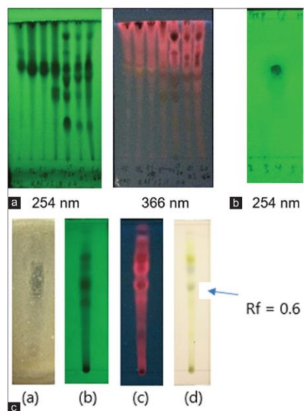
Figure 1: Thin layer chromatography profile of (a) Fraction D with mobile phase chloroform: Acetone: Formic acid (3:1:0.2); (b) Isolate (GLED2) using mobile phase n -hexane: Ethyl acetate (3:2); and (c) Contact bioautography profile of fraction D against bacillus subtilis . (a) the inoculated agar medium after the thin layer chromatography plate was removed (b) inspected thin layer chromatography under UV 254 nm (c) inspected thin layer chromatography under UV 366 nm (d) Inspected thin layer chromatography under visible light. (b) shows the pure compound using eluent n -hexane and ethyl acetate (3:2), having an Rf value of 0.6. This Rf value follows the bioautography result of the fraction D extract of ethyl acetate leaves (c). In the thin layer chromatography contact bioautographic assay, the eluted and dried thin layer chromatography plate transferred to Petri plate containing the agar medium has been inoculated with bacillus subtilis for approximately one hour and then incubated for 24 hours. Inhibition zones were detected in the spot with an Rf value of 0.6 on agar medium in a petri dish ((a) of c) after incubation, and the thin layer chromatography plate was removed. This showed that the isolate was active against bacillus subtilis .
