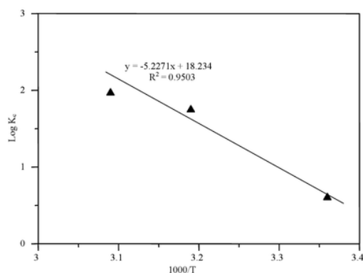
Figure 13. Van't Hoff's plots, \log K_c vs. 1000/T
