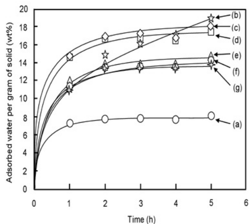
Figure 6 Percentage of adsorbed water on the surface of (a) Coal, (b) SO 3 H/Coal, (c) Ti(500)-SO 3 H/Coal, (d) Ti(1000)-SO 3 H/Coal, (e) Ti(1500)-SO 3 H/Coal, (f) Ti(2000)-SO 3 H/Coal and (g) Ti(2500)-SO 3 H/Coal
