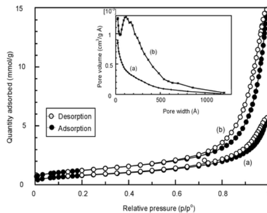
Figure 9 N 2 adsorption isotherms and pore size distribution of (a) Ti(2500)-SO 3 H/Coal and (b) Ti(2500)-SO 3 H/Coal500
