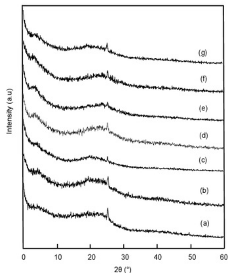
Figure 1 XRD patterns of (a) Coal, (b) SO 3 H/Coal, (c) Ti(500)-SO 3 H/Coal, (d) Ti(1000)-SO 3 H/Coal, (e) Ti(1500)-SO 3 H/Coal, (f) Ti(2000)-SO 3 H/Coal and (g) Ti(2500)-SO 3 H/Coal
