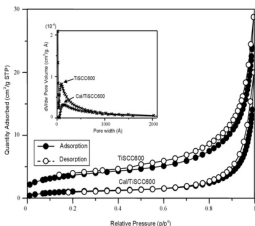
Figure 3. BET Surface Area of TiSCC600 and Cal/TiSCC600
