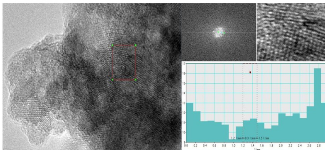
Figure 5. TEM image of TiSCC600
