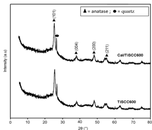
Figure 1. XRD pattern of TiSCC600 and Cal/TiSCC600
