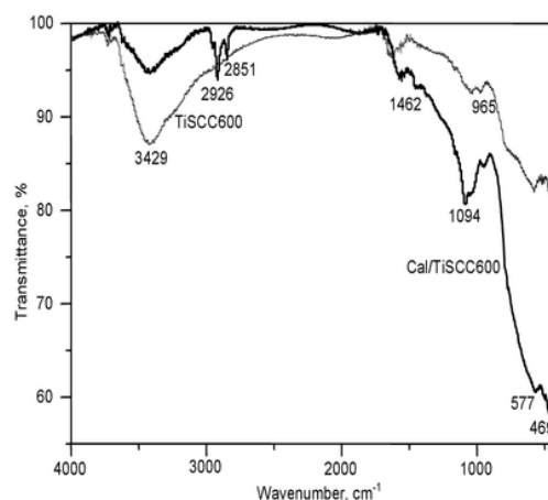
Figure 2. FTIR spectra of TiSCC600 and Cal/TiSCC600
