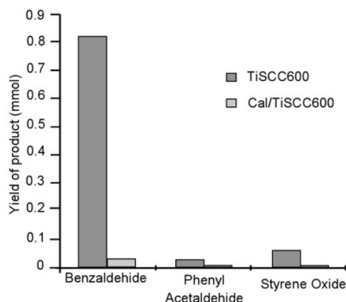
Figure 6. Comparison of catalytic activity of TiSCC600 and Cal/TiSCC600 in the oxidation of styrene (5 mmol), 30% \text{H}_2\text{O}_2 (5 mmol) and catalyst (50 mg). The yield of product at room temperature for 20 h
