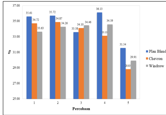
Figure 5 Fixed Carbon Graph
