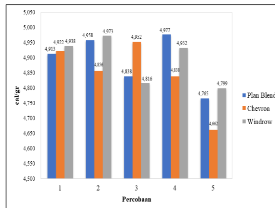
Figure 7 calorific Value Graph
