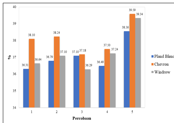
Figure 4 Volatile Matter Graph
