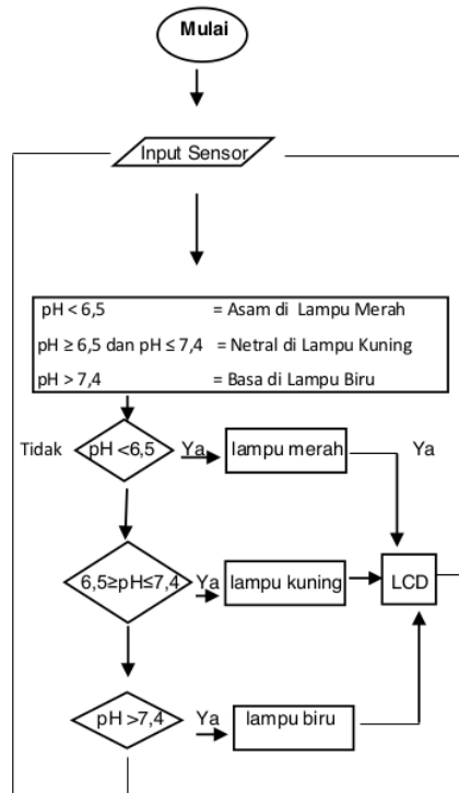
Gambar 1. Flowchart sistem
