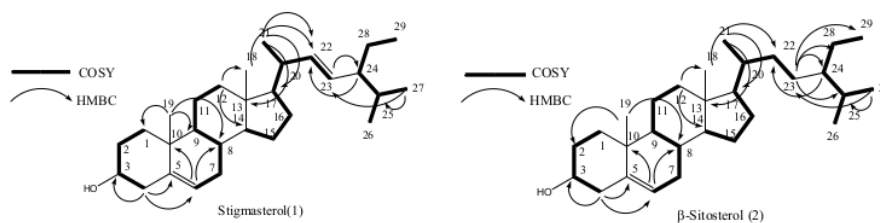
Fig.-1: Chemical Structure of Stigmasterol (1) and \beta -Sitosterol (2)
