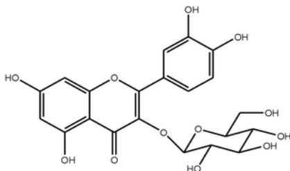
Fig. 3: Chemical structure of compound (3) 3-O- \beta -D-glucopyranoside or isoquercetin.
