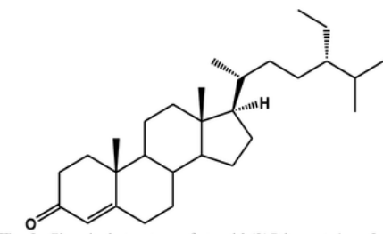
Fig. 2: Chemical structure of steroid (2) Stigmast-4-en-3-one.
