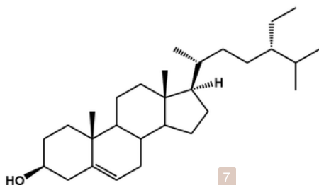
Fig. 1: Chemical structure of steroid (1) stigmast-5(6)-en-3 \beta -ol or \beta -sitosterol.
