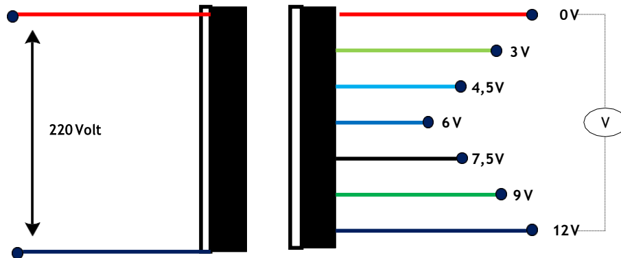
Gambar 2.1. Transformator
