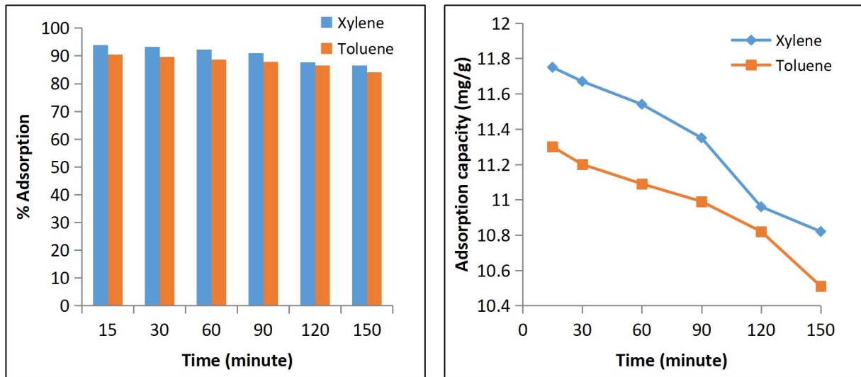
Figure 6. % Adsorption and Adsorption Capacity (SBA-15 mass = 0.1 grams, concentration of toluene and xylene = 25 mg/L)
