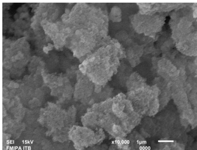
Figure 4. SEM picture of SBA-15 material from rice husk ash
