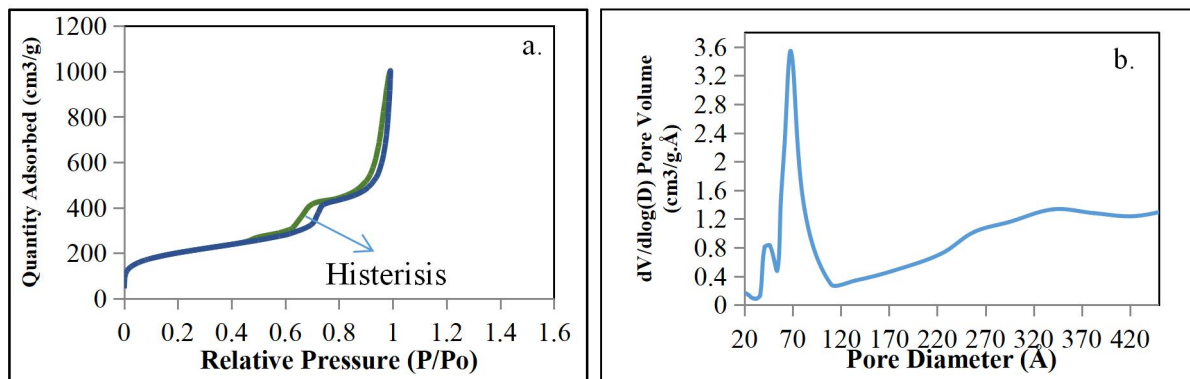
Figure 1. a. N 2 adsorption / desorption isotherm, b. Pore distribution of SBA-15 material from rice husk ash
