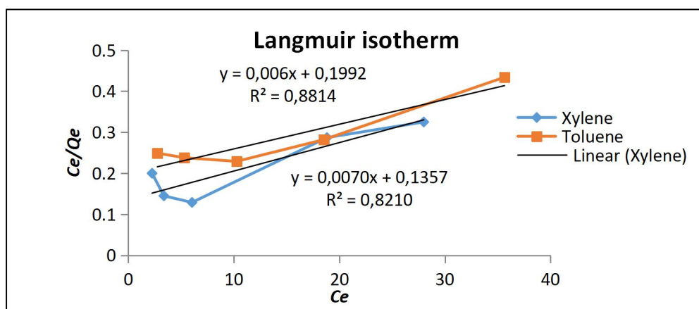
Figure 7. Langmuir Isotherm Graph
