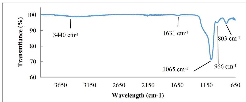
Figure 3. FTIR spectrum of SBA-15 material from rice husk ash
