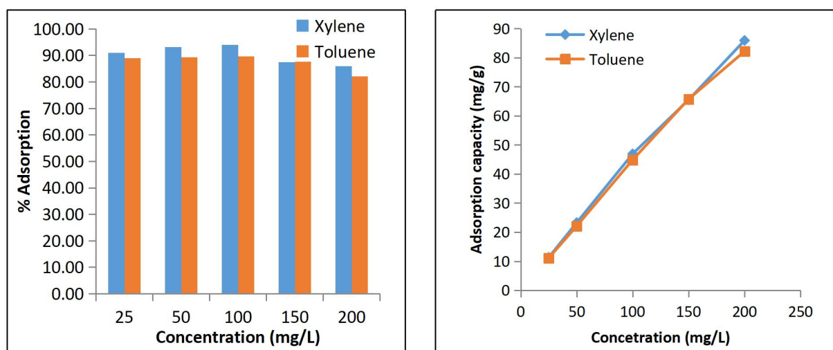
Figure 5. % Adsorption and Adsorption Capacity of toluene and xylene with SBA-15 from rice husk ash (SBA-15 mass = 0.1 grams, adsorption time = 60 minutes)
