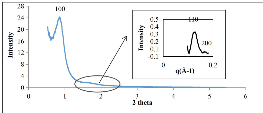
Figure 2. SAXS Pattern of SBA-15 Rice Husk Ash
