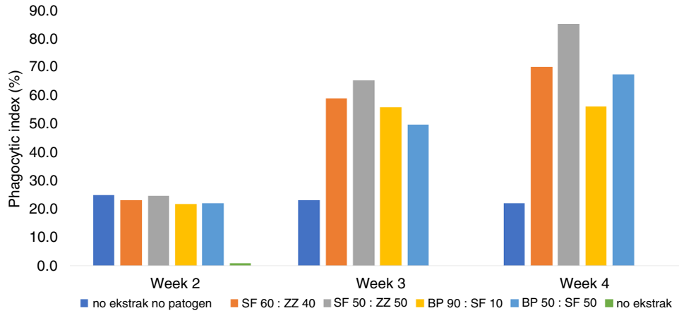
Figure 1. Phagocytic index (%) of Tilapia ( Oreochromis niloticus ) fed different extract combination in treatment trials. BP, Boesenbergia pandurata ; SF, Solanum ferox ; ZZ, Zingiber zerumbet .
