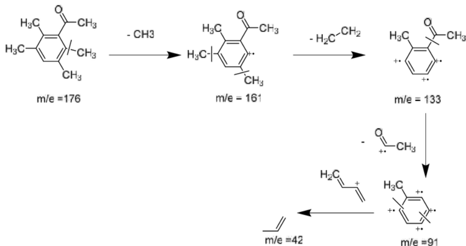
Gambar 4. Pola Fragmentasi senyawa 1-(2,3,5,6-Tetramethylphenyl) Ethanone
