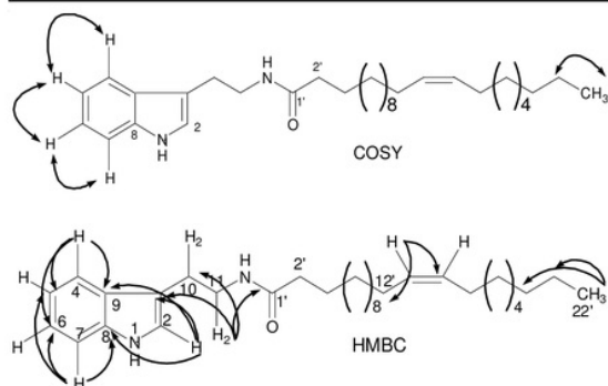
Fig. 2. Significant COSY and HMBC correlation of compound 1
