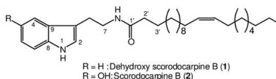
Fig. 1. Chemical structure of scorodocarpine alkaloids
