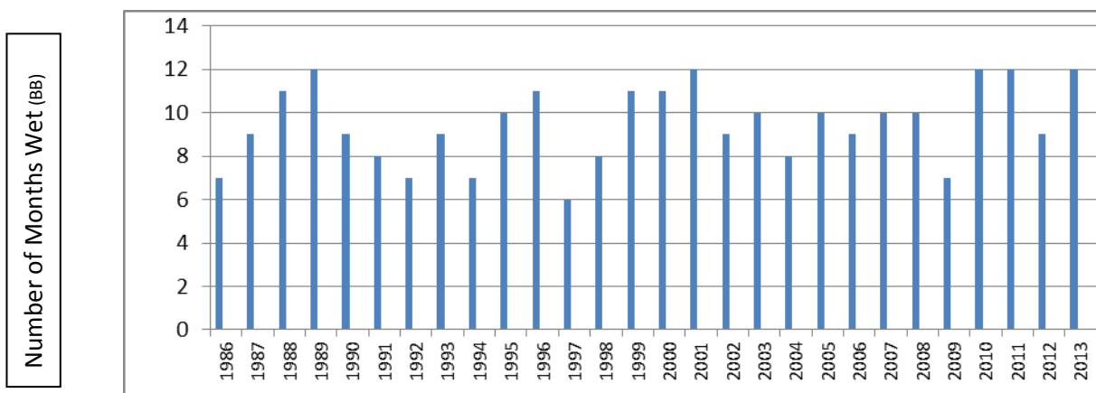
Figure 4. A number of the wet seasons (months in a year) started from 1986 to 2013 in Bangun city.
