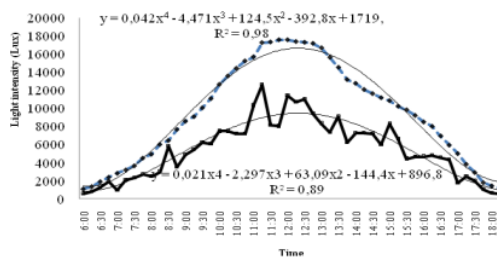
Figure 7. Light intensity on calliandra ( Calliandra calothyrsus ) shading
