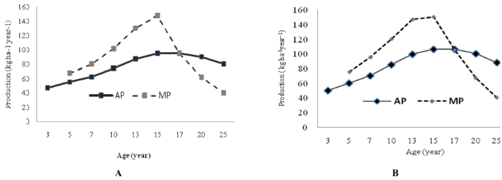
Figure 17. Correlation between average annual production (AP) and average on-going annual production or marginal product (MP) of Arabica coffee under lamtoro ( Leucaena glauca ) (left) and calliandra ( Calliandra calothyrsus ) (right) shading
