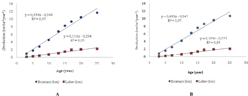
Figure 10. Biomass and brown-waste matter on: A. Lamtoro ( Leucaena glauca ), B. Calliandra ( Calliandra calothyrsus ) shadings
