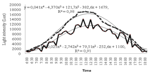
Figure 8. Light intensity on lamtoro ( Leucaena glauca ) shading
