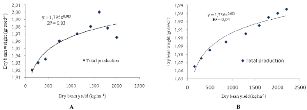
Figure 18. Arabica coffee bean total production and bean dry weight produced under lamtoro ( Leucaena glauca ) (left) and calliandra ( Calliandra calothyrsus ) (right) shading
