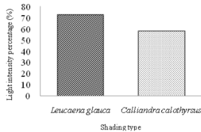
Figure 9. Light intensity percentage on calliandra ( Calliandra calothyrsus ) and lamtoro ( Leucaena glauca ) shading types
