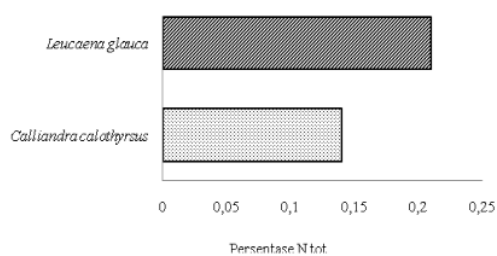
Figure 13. Total N content on calliandra ( Calliandra calothyrsus ) and lamtoro ( Leucaena glauca ) shadings
