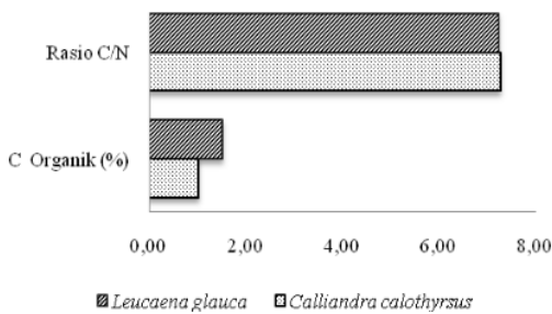
Figure 14. Macronutrients content on calliandra ( Calliandra calothyrsus ) and lamtoro ( Leucaena glauca ) shadings
