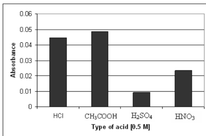
Fig. 5. Effect of acid type towards Sn(II) determination with HG-QFAAS method
