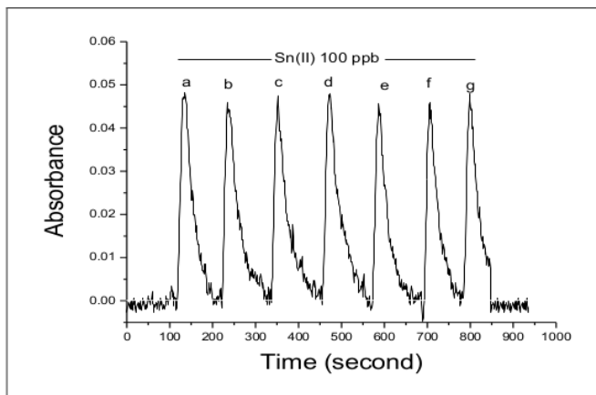
Fig. 9. Analytical signal profile for 100 ppb Sn(II) reproducibility at various measurement
