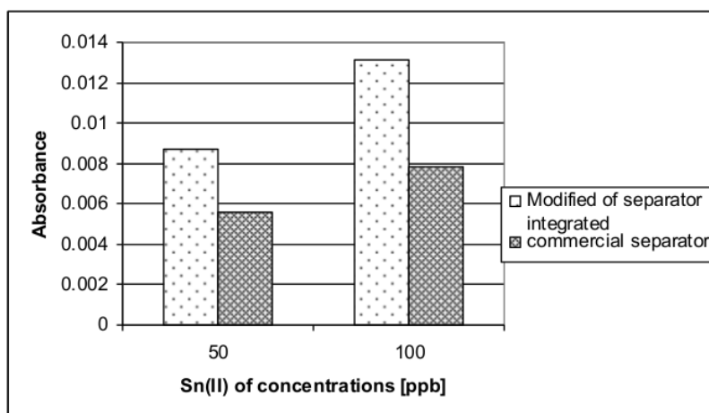
Fig. 10. Comparison of gas-liquid separator integrated and commercial separator
