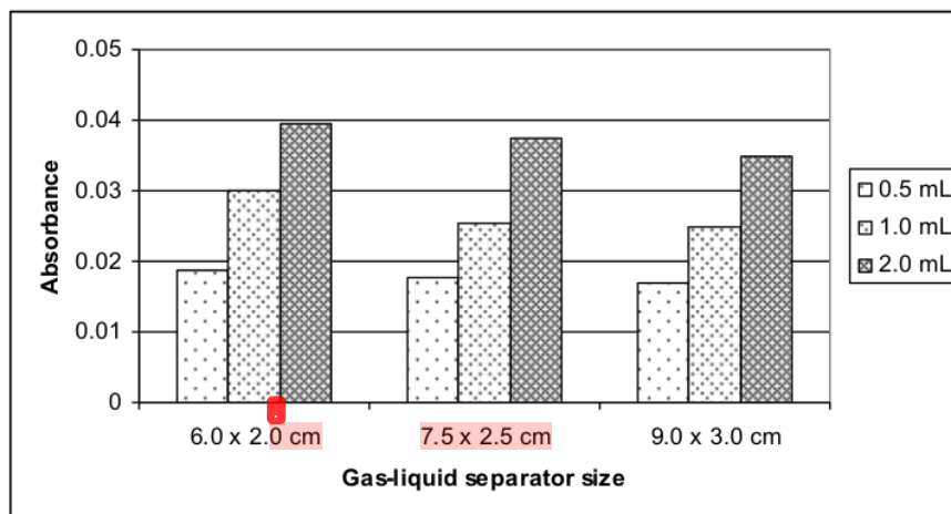
Fig. 4. Absorbance curve of Sn(II) standard at mixing system in gas-liquid separator
