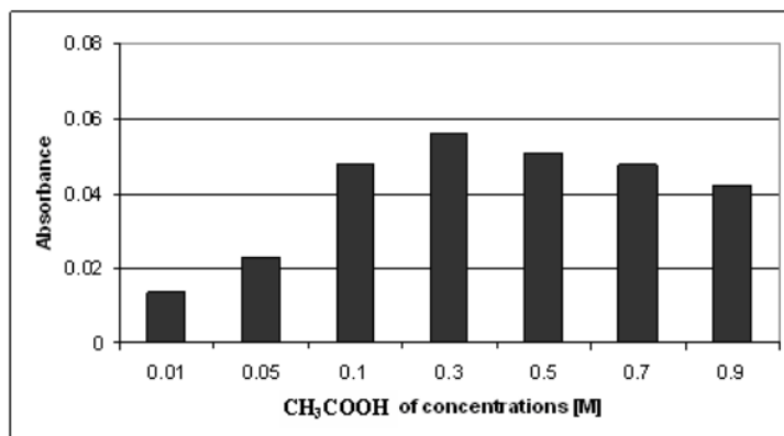
Fig. 6. Effect of CH 3 COOH concentration in Sn(II) determination with HG-QFAAS method
