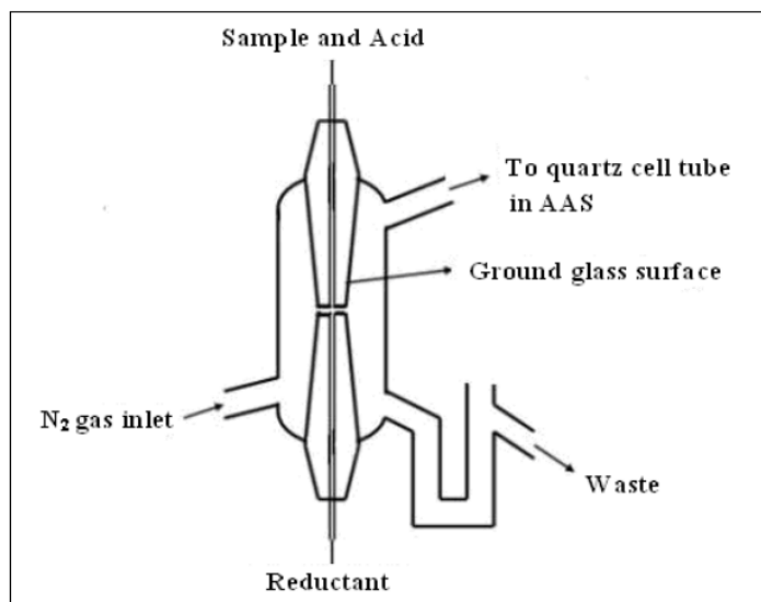
Fig. 1. Gas-liquid Separator hydride generator
