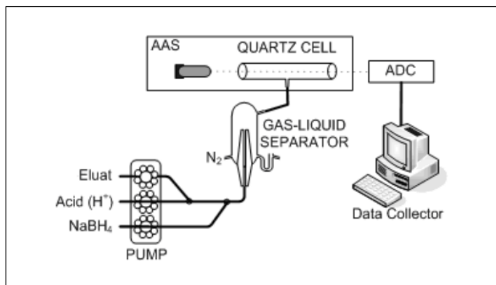
Fig.2. Equipment of the HG-QFAAS system
