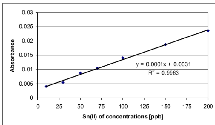
Fig. 8. Calibration curve Sn(II) for determination with HG-QFAAS method
