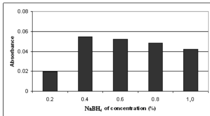
Fig. 7. Effect of NaBH 4 concentration in Sn(II) determination with HG-QFAAS method
