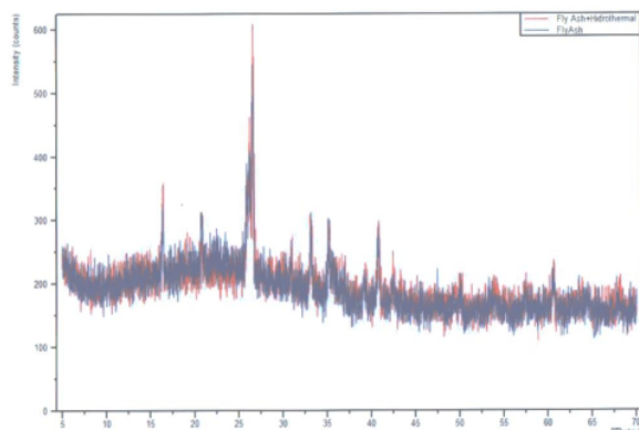
Figure 3. Combining the diffractograms (Red : Fly ash + Hidrotermal, Blue : Fly ash)
