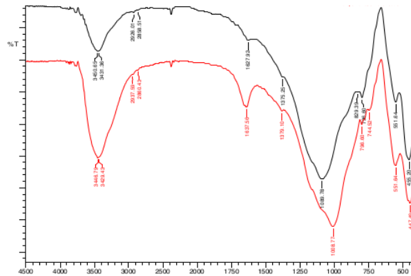
Figure 5. FTIR Spectrum of Fly Ash and Synthetic Zeolite
