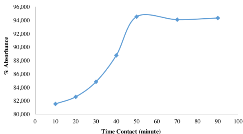
Figure 9. The curve of synthetic zeolite contact time variation on \text{Cu}^{2+} ion absorbance
