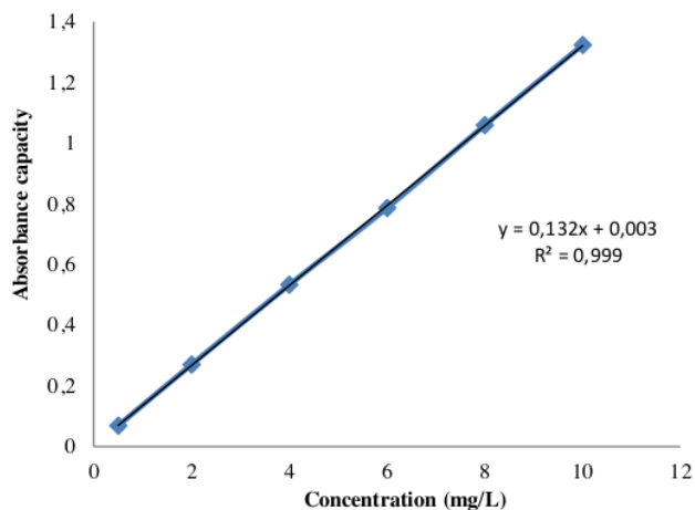
Figure 6. Cu standard curve
