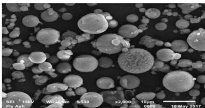
Figure 1. Surface morphology of fly ash, 2000x magnification
