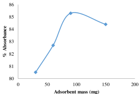
Figure 12. Fly ash weight curve against \text{Cu}^{2+} ion adsorption
