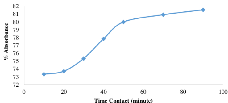
Figure 10. The curve of fly ash contact time variation on \text{Cu}^{2+} ion absorbance
