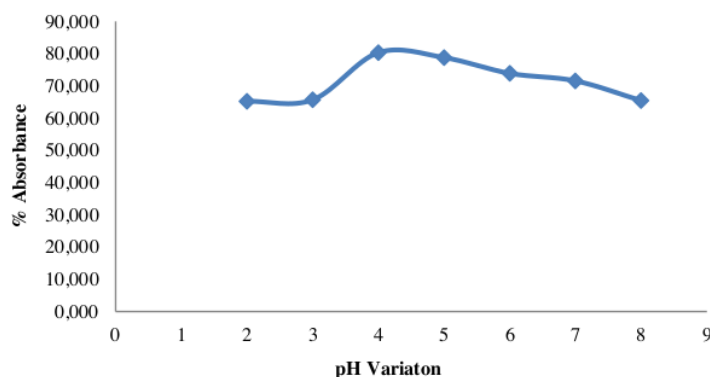
Figure 7. Influence Curve of Synthetic Zeolite pH on \text{Cu}^{2+} ion absorption
