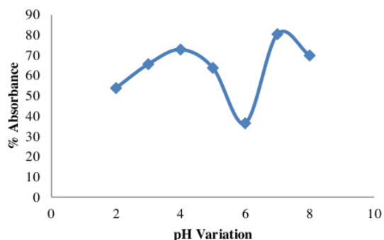
Figure 8. The curve of the effect of fly ash pH on the absorption of \text{Cu}^{2+} ions
