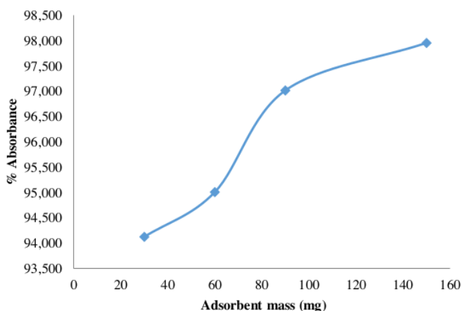
Figure 11. Synthetic zeolite weight curve for \text{Cu}^{2+} ion adsorption
