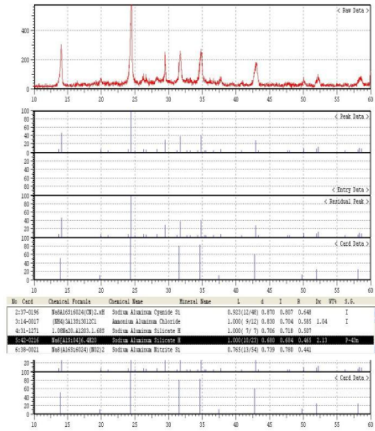
Figure 4. Characterization of the XRD database
