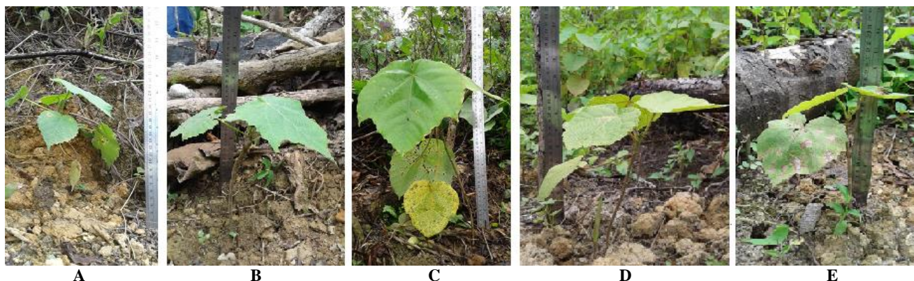
Figure 3. Macaranga gigantea at planting plots (four months), with application organic manure: A. P0 (0 g), B. P1 (100 g), C. P2 (200 g), D. P3 (300 g), E. P4 (400 g) for each plant
