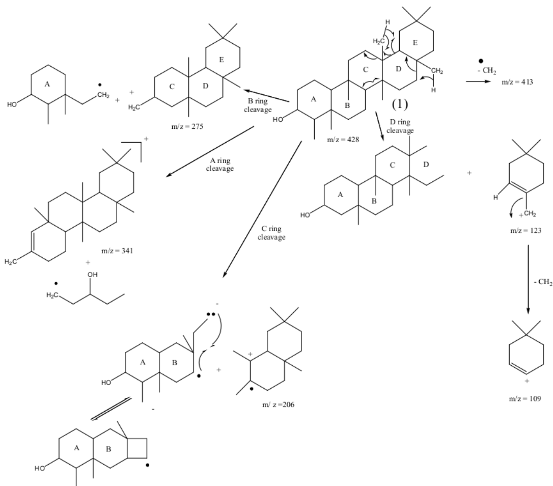
Figure 3 Mass Fragmentation Pattern of Compound 1
