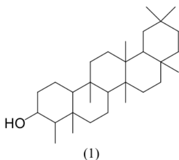
Figure 1 Friedelinol
