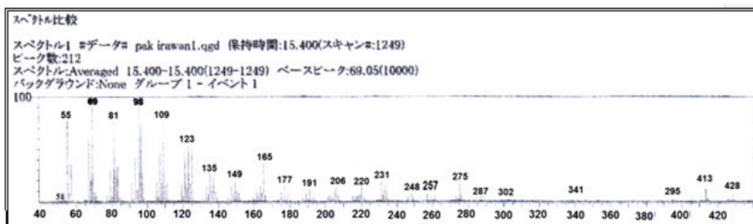
Figure 2 MS spectrum of friedelinol
