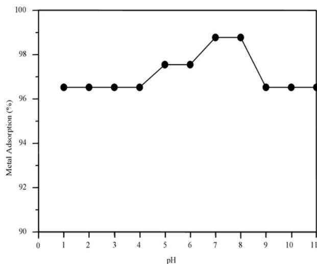
Figure 7. The Effect of pH to Metal Adsorption
