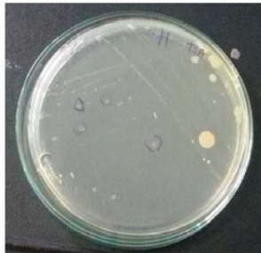
Figure 3. Bacteria Edwardsiella ictaluri colonies isolated from Pangasius pangasius on TSA medium after 48 hours incubation. The bacteria collected from internal organs were streaked on TSA medium and afterward incubated at 28°C for 48 hours. The colonies of bacteria are good growth. The morphology of colonies of bacteria dominant was smooth, white, uniform. The average diameter of the colonies is 0.15 mm. That bacteria colony is more dominantly grow compared to other bacteria colony. In addition to that, other types of bacteria colony are also grown. Yellow colony in bigger size and white colony in medium size. The next identification process is by bacteria purification based on some different morphologies of colony. It shows that there are other bacteria types found in the fish samples.
