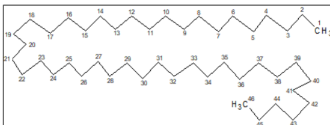
Figure 1 Hexa-tetra contana compound structure.
