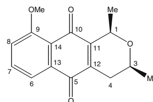
Fig. 1 Structure of compound 1 (eleutherin)
