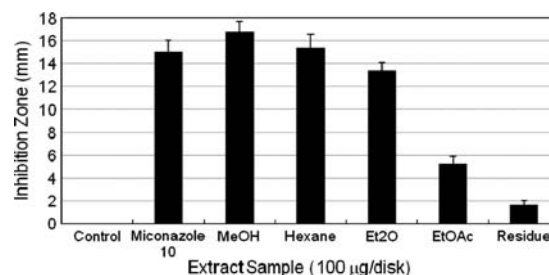
Fig. 2 Antidermatophyte activity of the methanolic extract and the soluble fractions from E. americana against T. mentagrophytes (all values are the mean of triplicates \pm standard deviation (SD))
